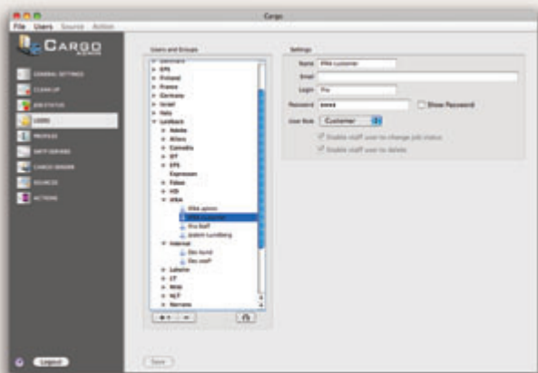
Cargo User admin interface
